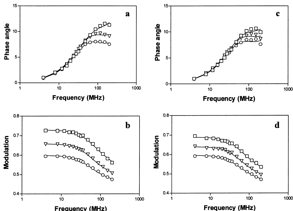
Fig. 2 Typical experimental traces of differential frequency response curves for holo-Cam38-Alexa488 (a, phase; b, modulation) and holo-Cam111-Alexa488 (c, phase; d, modulation) for the protein alone (squares), in the presence of the IQ3 peptide (triangles) and in the presence of IQ34 peptide (circles). The lines show fitted functions. See Materials and methods section for data collection and analysis
